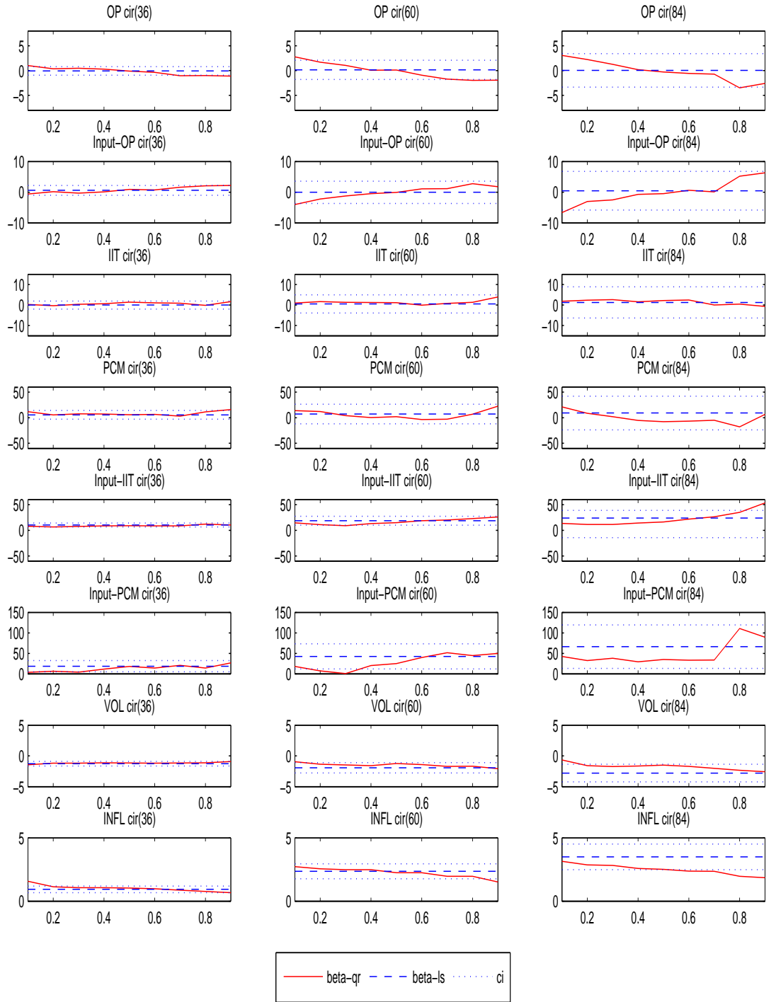
FIG 5. Quantile coefficient estimates.
