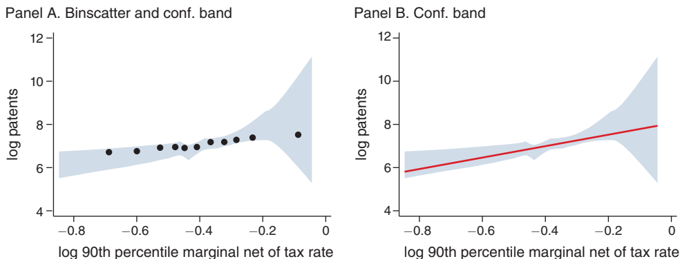
FIGURE 3. CONFIDENCE BANDS
