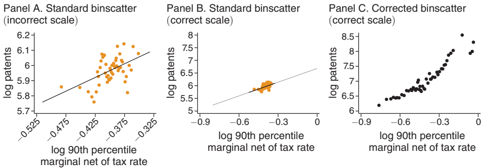
FIGURE 2. COVARIATE ADJUSTMENT
