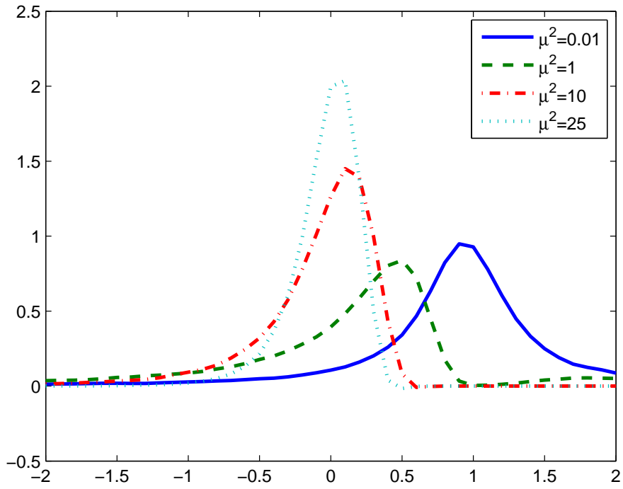
Figure 1: Finite-sample distribution of the TLS estimator given by formula (4) for different values of the concentration parameter. \rho = 0.95 , \frac{\sigma_e}{\sigma_v} = 1 , \beta_0 = 0 , r = 1
